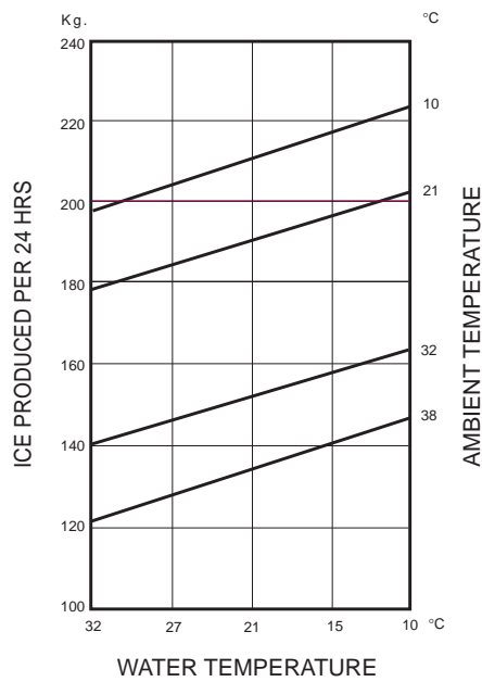
AIR COOLED MODELS
