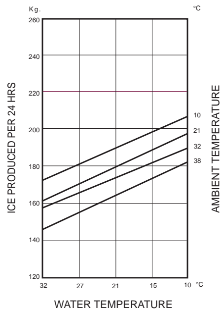
WATER COOLED MODELS
